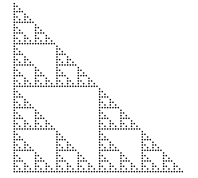
Figure 2. Draw sierpinski .
